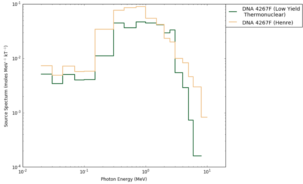
Figure 6. Photon spectra from thermonuclear sources
